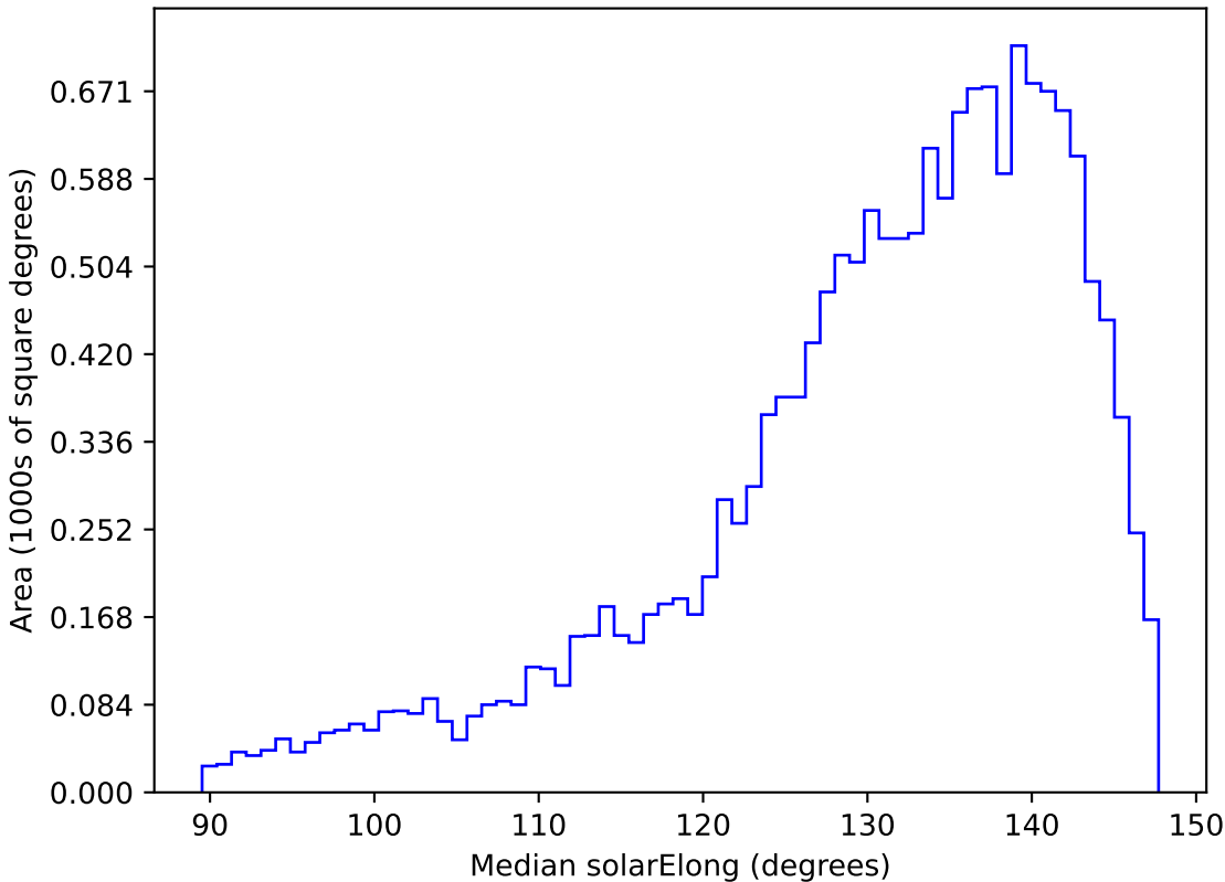
too_elab_r128_d2_griz_v3.4_10yrs WFD r band: Median solarElong
