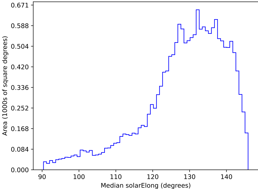
too_elab_r128_d2_griz_v3.4_10yrs WFD i band: Median solarElong
