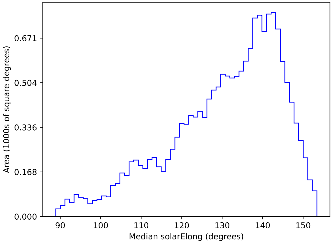
too_elab_r128_d2_griz_v3.4_10yrs WFD g band: Median solarElong
