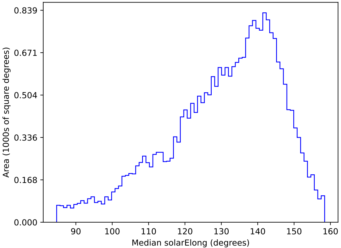
too_elab_r128_d2_griz_v3.4_10yrs All sky g band: Median solarElong
