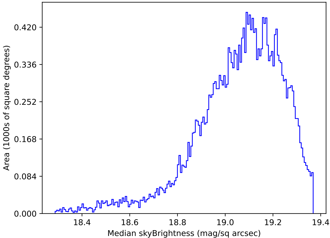
too_elab_r128_d2_griz_v3.4_10yrs Yr 1 z band: Median skyBrightness
