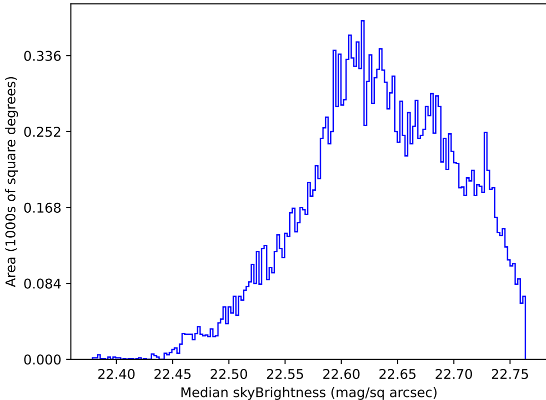
too_elab_r128_d2_griz_v3.4_10yrs Yr 1 u band: Median skyBrightness
