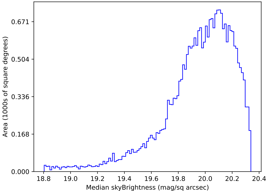
too_elab_r128_d2_griz_v3.4_10yrs Yr 1 i band: Median skyBrightness
