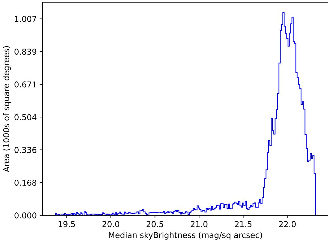
too_elab_r128_d2_griz_v3.4_10yrs Yr 1 g band: Median skyBrightness
