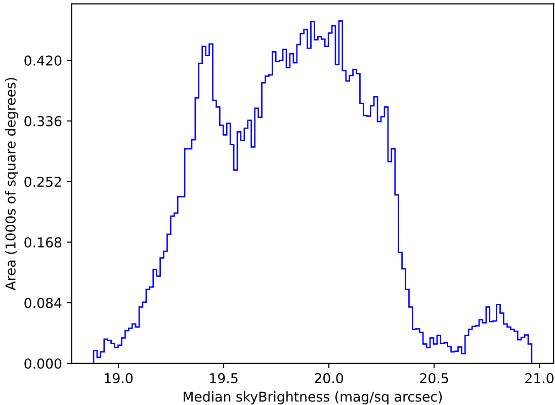
too_elab_r128_d2_griz_v3.4_10yrs Yr 1 all bands: Median skyBrightness
