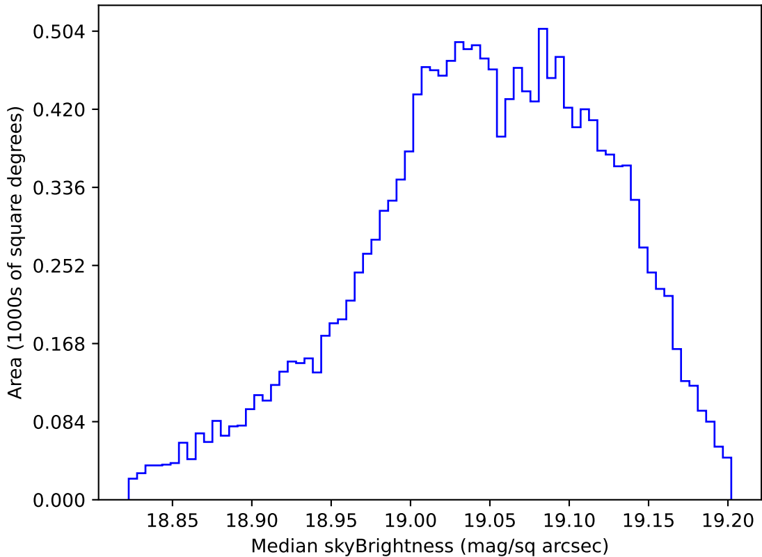
too_elab_r128_d2_griz_v3.4_10yrs WFD z band: Median skyBrightness
