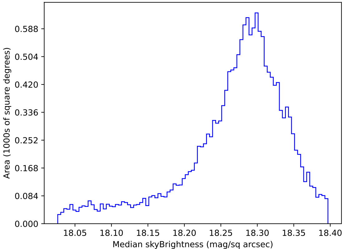
too_elab_r128_d2_griz_v3.4_10yrs WFD y band: Median skyBrightness
