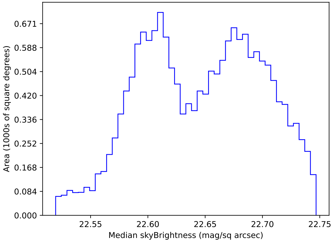
too_elab_r128_d2_griz_v3.4_10yrs WFD u band: Median skyBrightness
