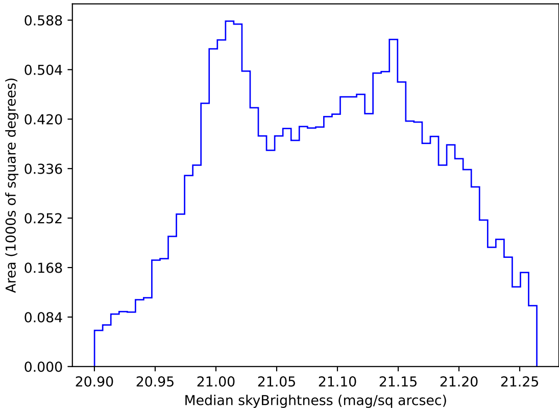
too_elab_r128_d2_griz_v3.4_10yrs WFD r band: Median skyBrightness
