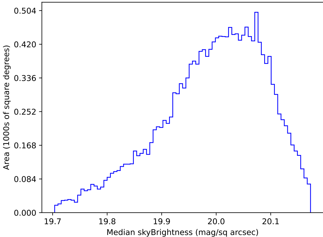
too_elab_r128_d2_griz_v3.4_10yrs WFD i band: Median skyBrightness
