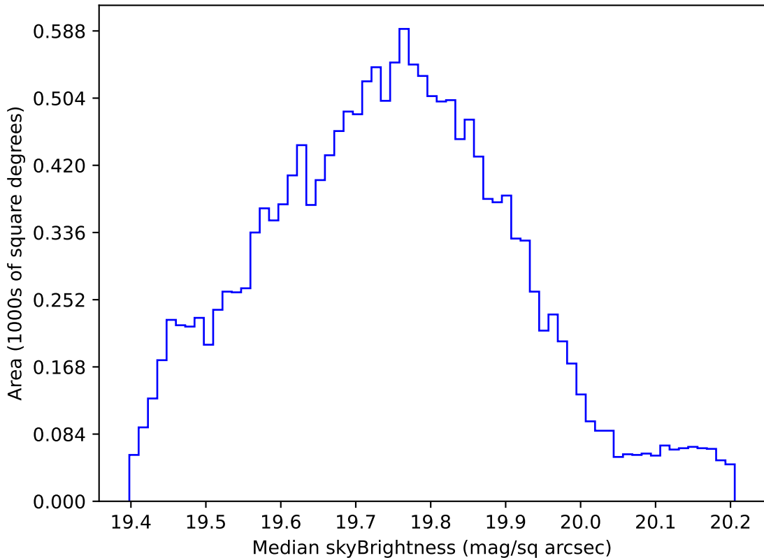
too_elab_r128_d2_griz_v3.4_10yrs WFD all bands: Median skyBrightness
