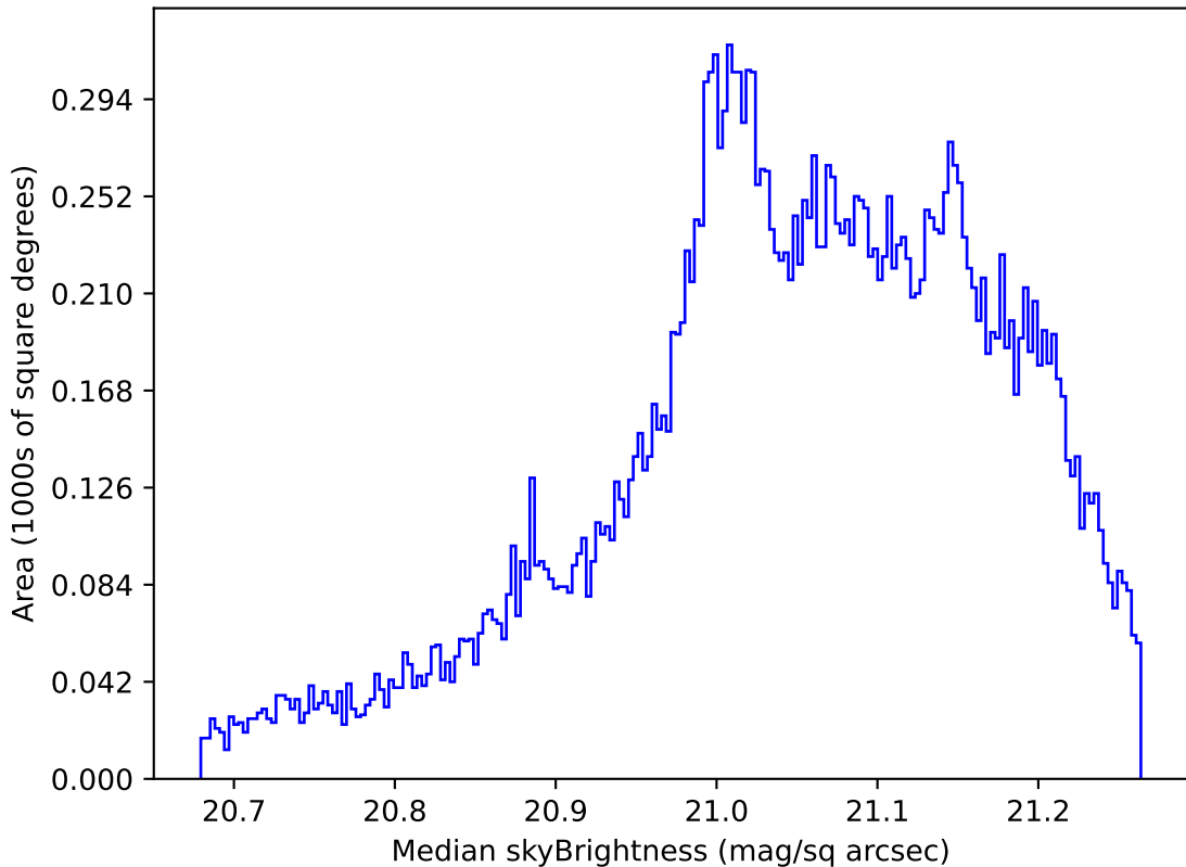
too_elab_r128_d2_griz_v3.4_10yrs All sky r band: Median skyBrightness
