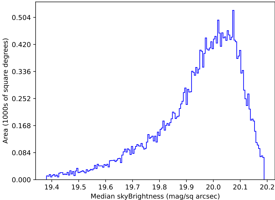
too_elab_r128_d2_griz_v3.4_10yrs All sky i band: Median skyBrightness
