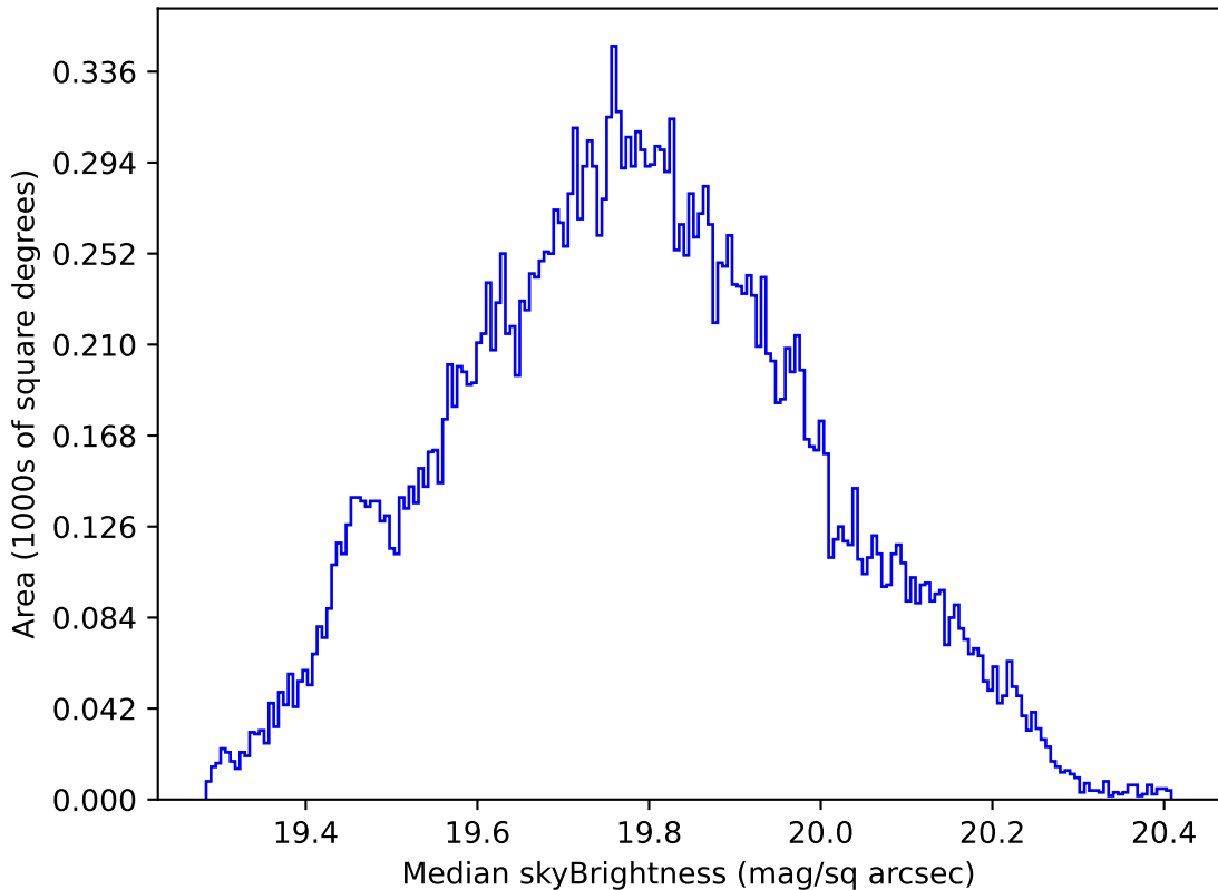
too_elab_r128_d2_griz_v3.4_10yrs All sky all bands: Median skyBrightness
