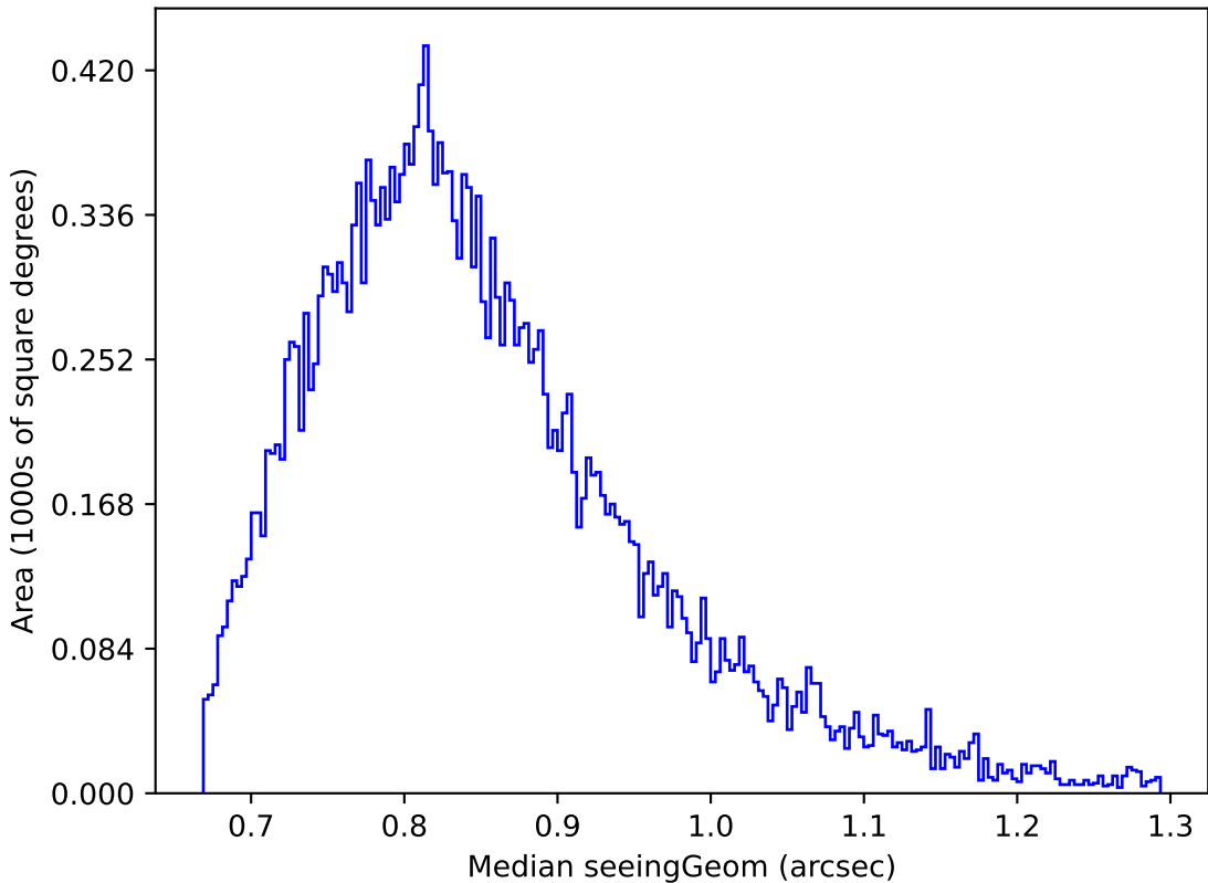
too_elab_r128_d2_griz_v3.4_10yrs Yr 1 z band: Median seeingGeom
