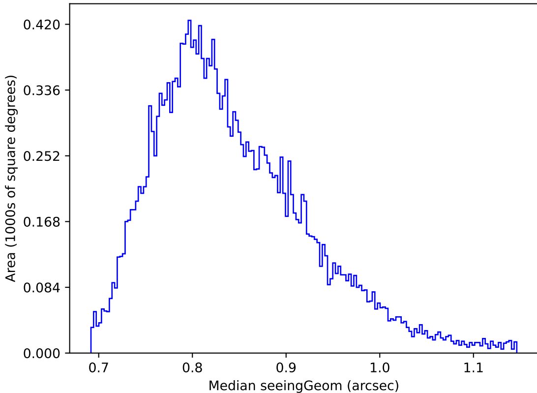
too_elab_r128_d2_griz_v3.4_10yrs Yr 1 y band: Median seeingGeom
