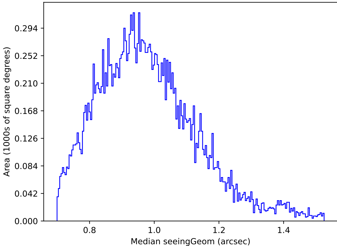
too_elab_r128_d2_griz_v3.4_10yrs Yr 1 u band: Median seeingGeom
