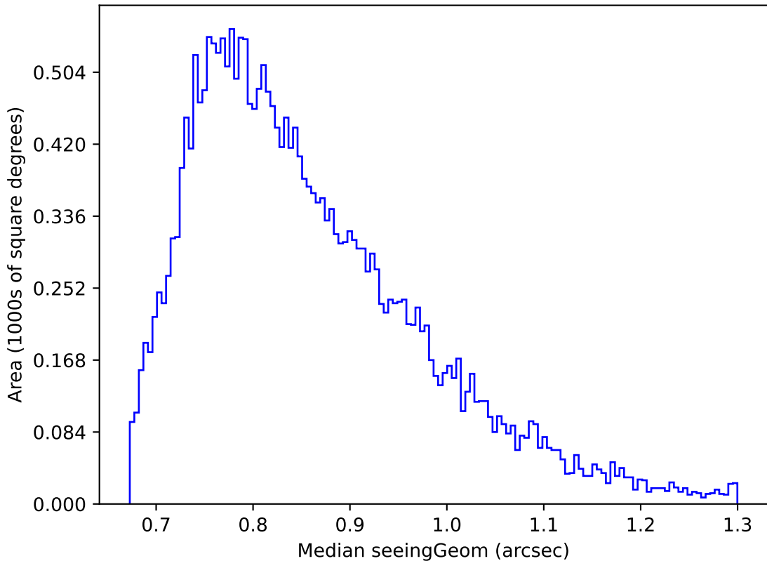
too_elab_r128_d2_griz_v3.4_10yrs Yr 1 r band: Median seeingGeom
