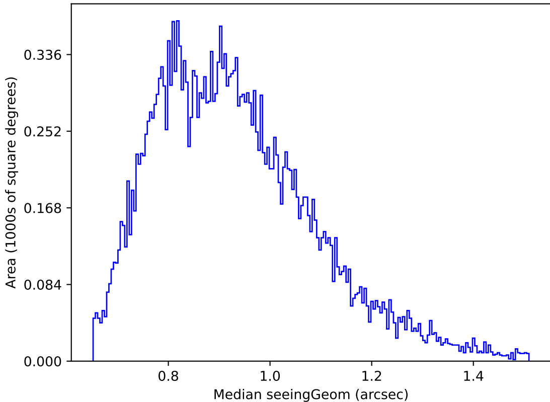
too_elab_r128_d2_griz_v3.4_10yrs Yr 1 g band: Median seeingGeom
