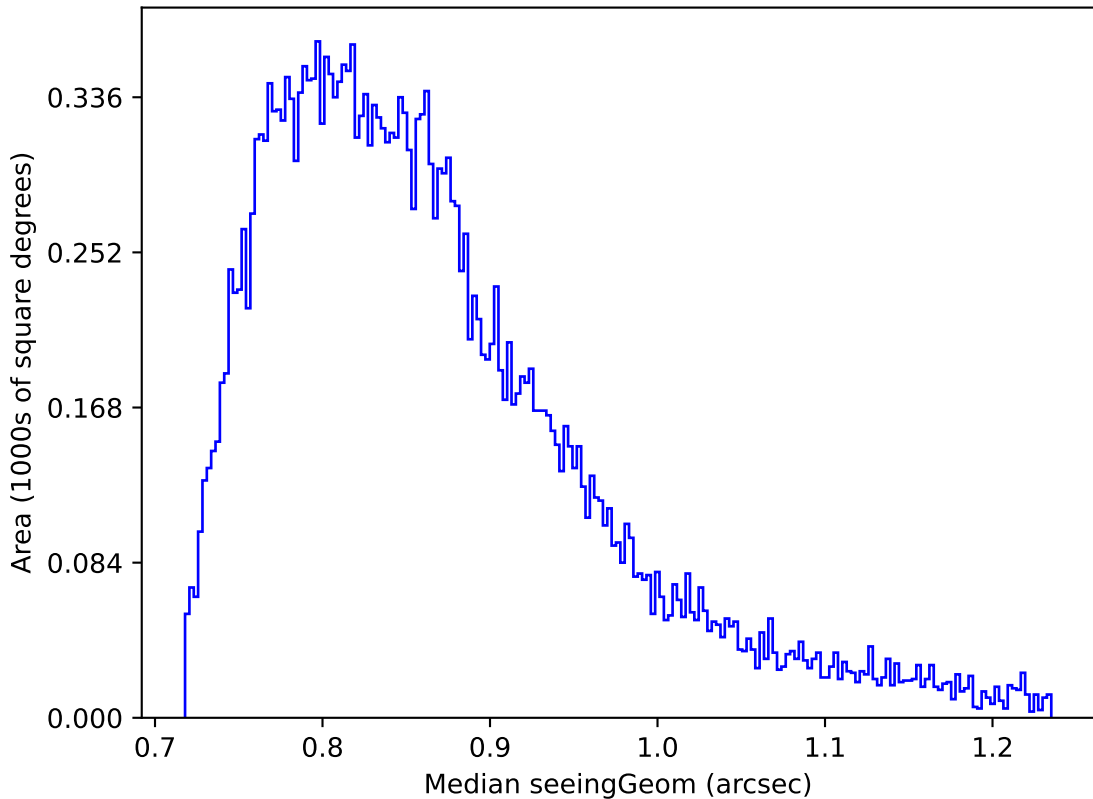
too_elab_r128_d2_griz_v3.4_10yrs Yr 1 all bands: Median seeingGeom
