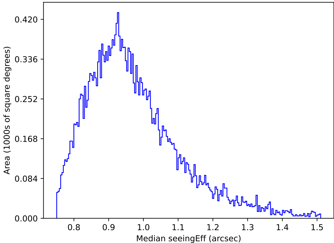
too_elab_r128_d2_griz_v3.4_10yrs Yr 1 z band: Median seeingEff
