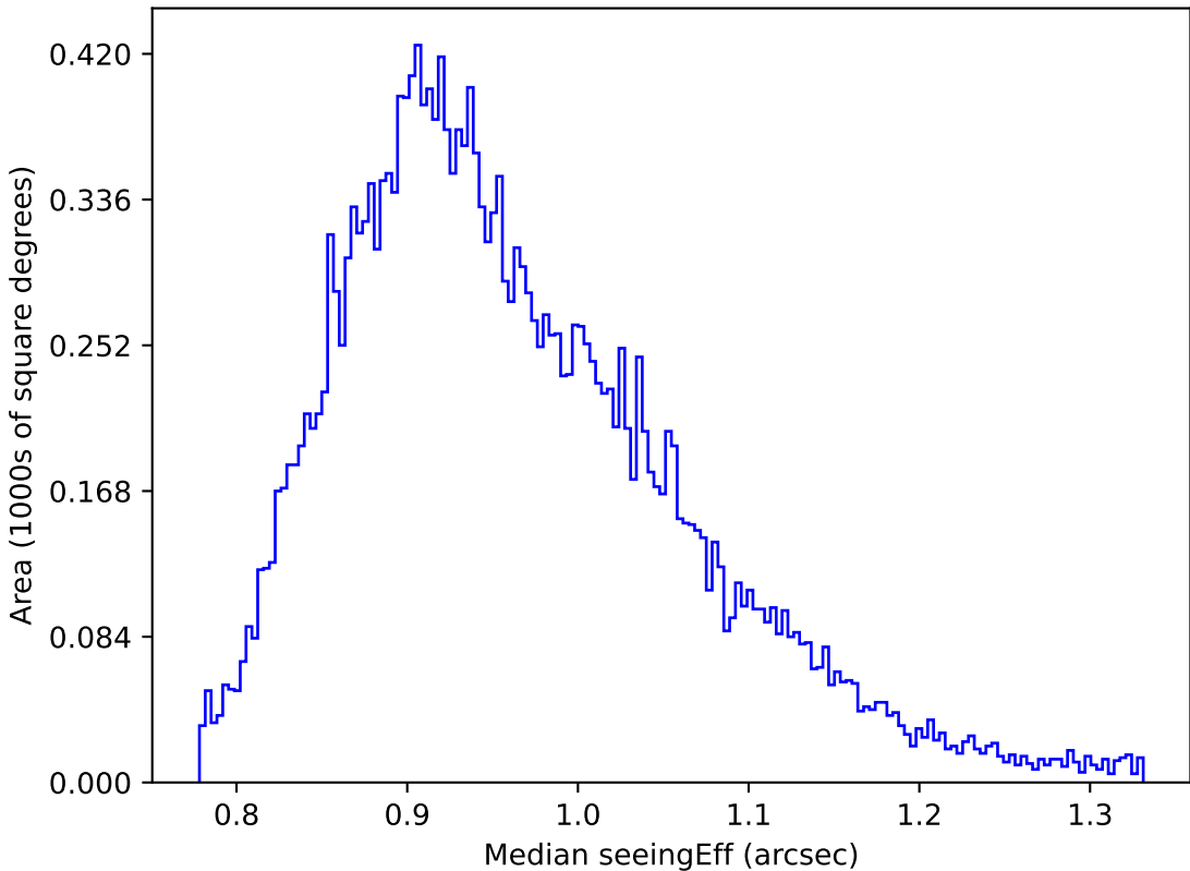
too_elab_r128_d2_griz_v3.4_10yrs Yr 1 y band: Median seeingEff
