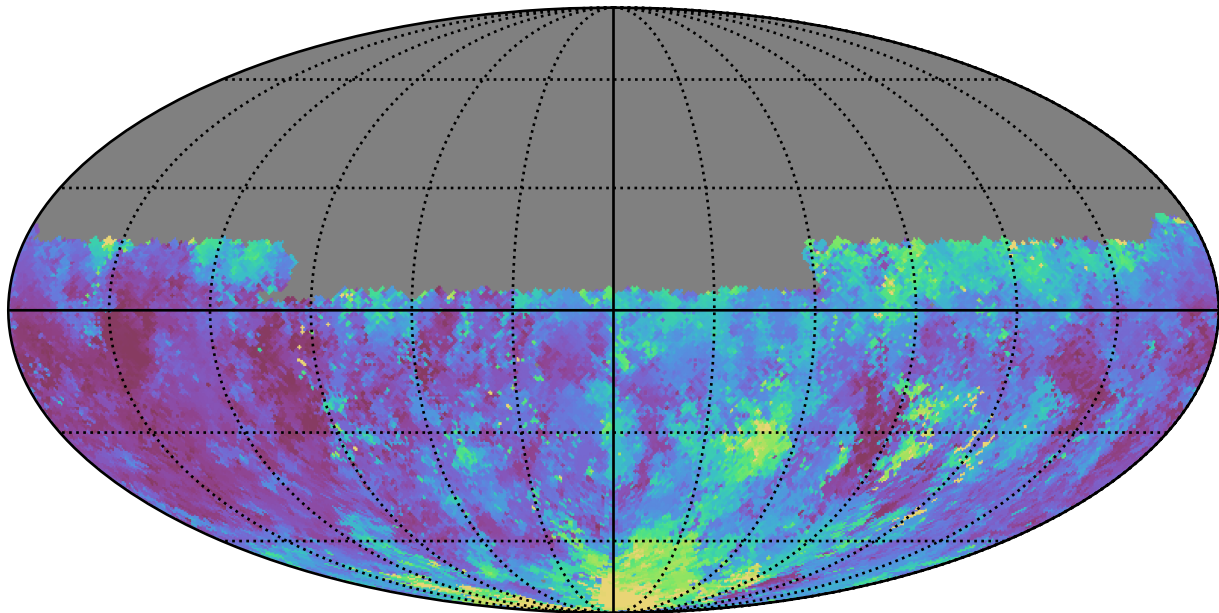
too_elab_r128_d2_griz_v3.4_10yrs Yr 1 u band: Median seeingEff
