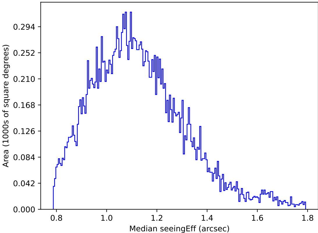
too_elab_r128_d2_griz_v3.4_10yrs Yr 1 u band: Median seeingEff
