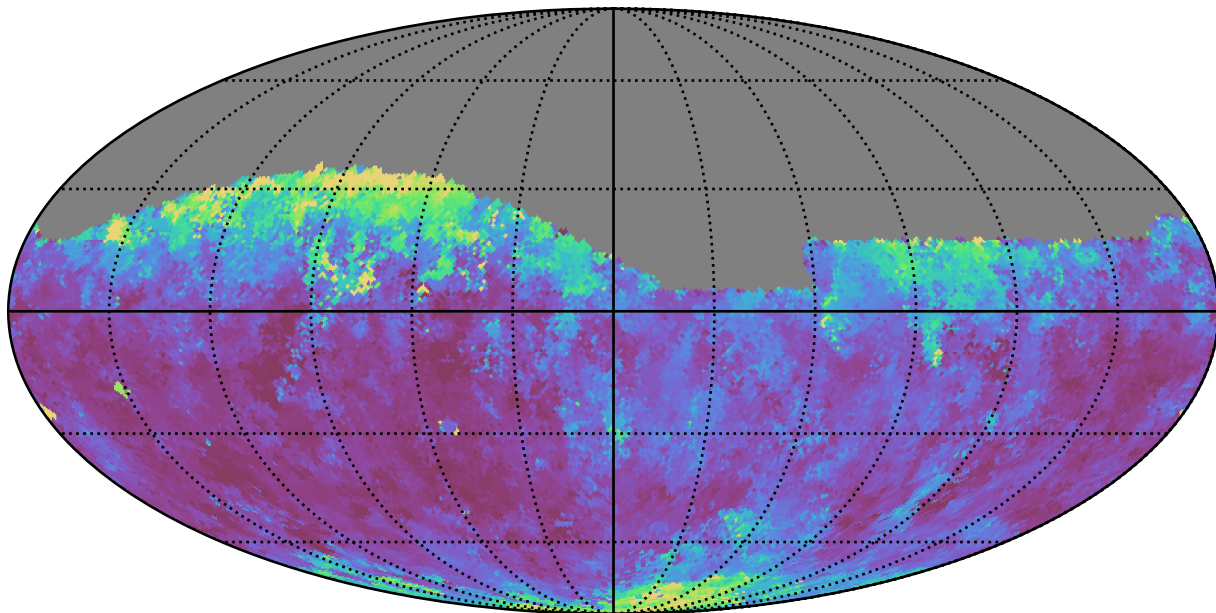
too_elab_r128_d2_griz_v3.4_10yrs Yr 1 i band: Median seeingEff
