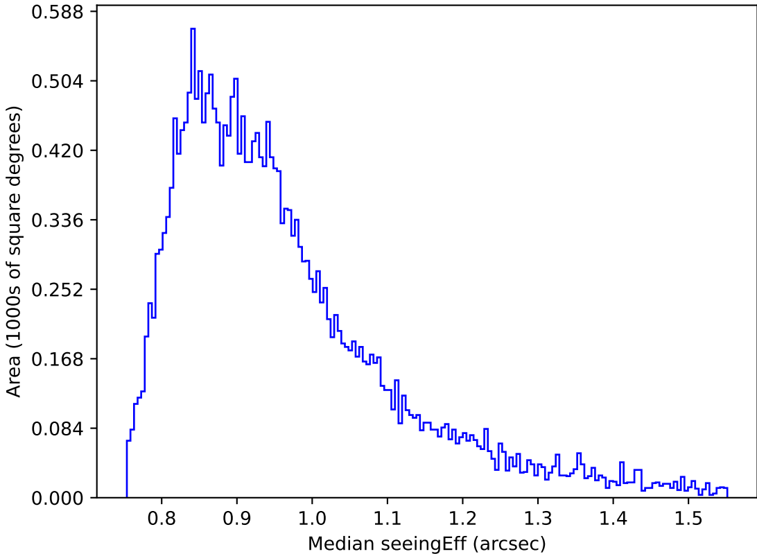
too_elab_r128_d2_griz_v3.4_10yrs Yr 1 i band: Median seeingEff
