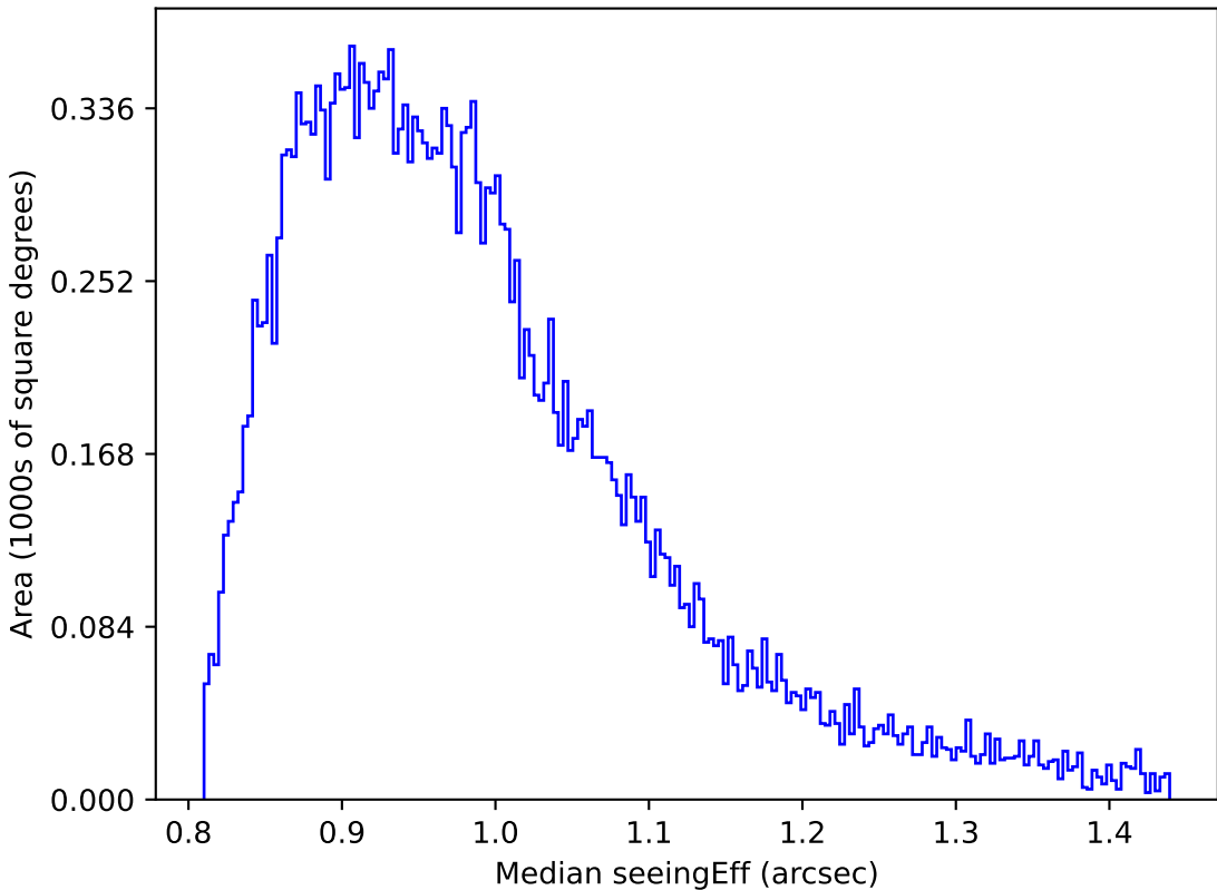
too_elab_r128_d2_griz_v3.4_10yrs Yr 1 all bands: Median seeingEff
