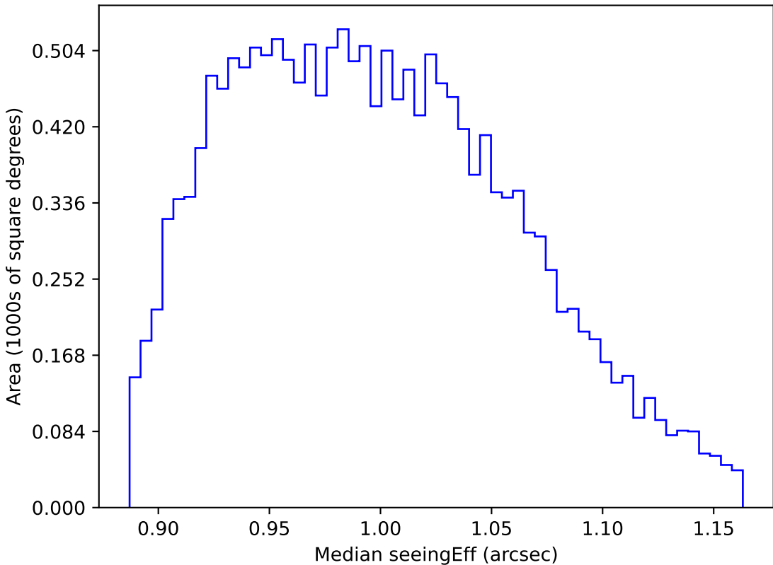
too_elab_r128_d2_griz_v3.4_10yrs WFD y band: Median seeingEff
