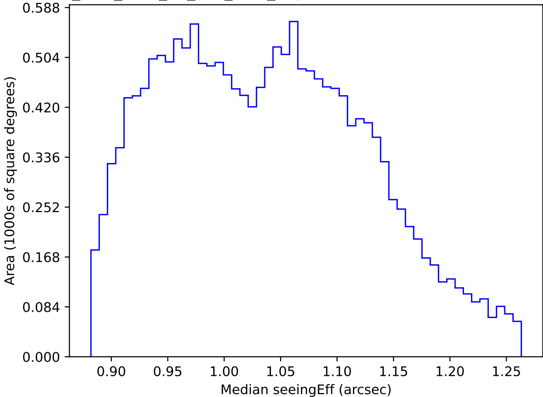
too_elab_r128_d2_griz_v3.4_10yrs WFD r band: Median seeingEff
