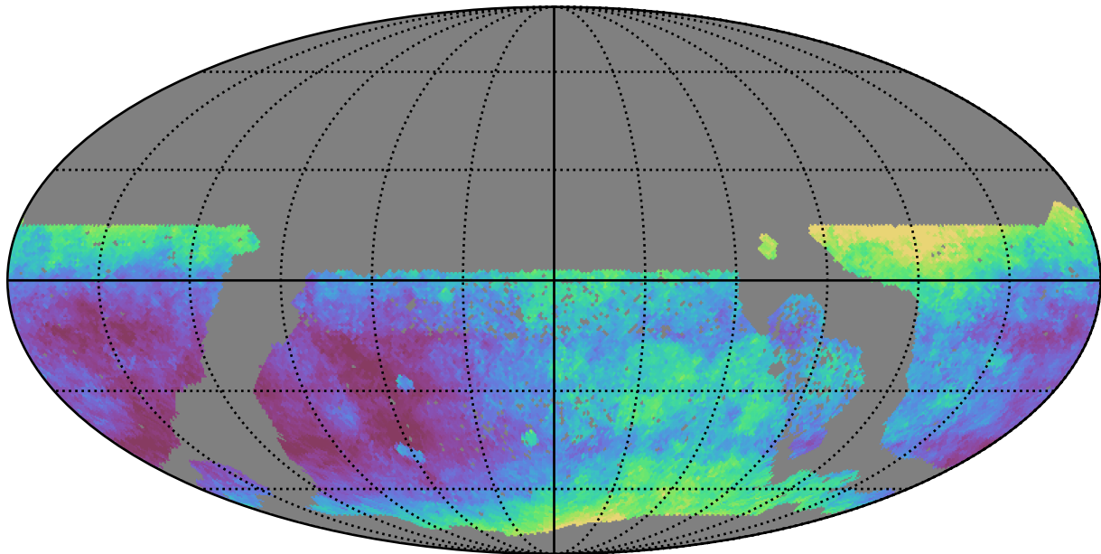
too_elab_r128_d2_griz_v3.4_10yrs WFD i band: Median seeingEff
