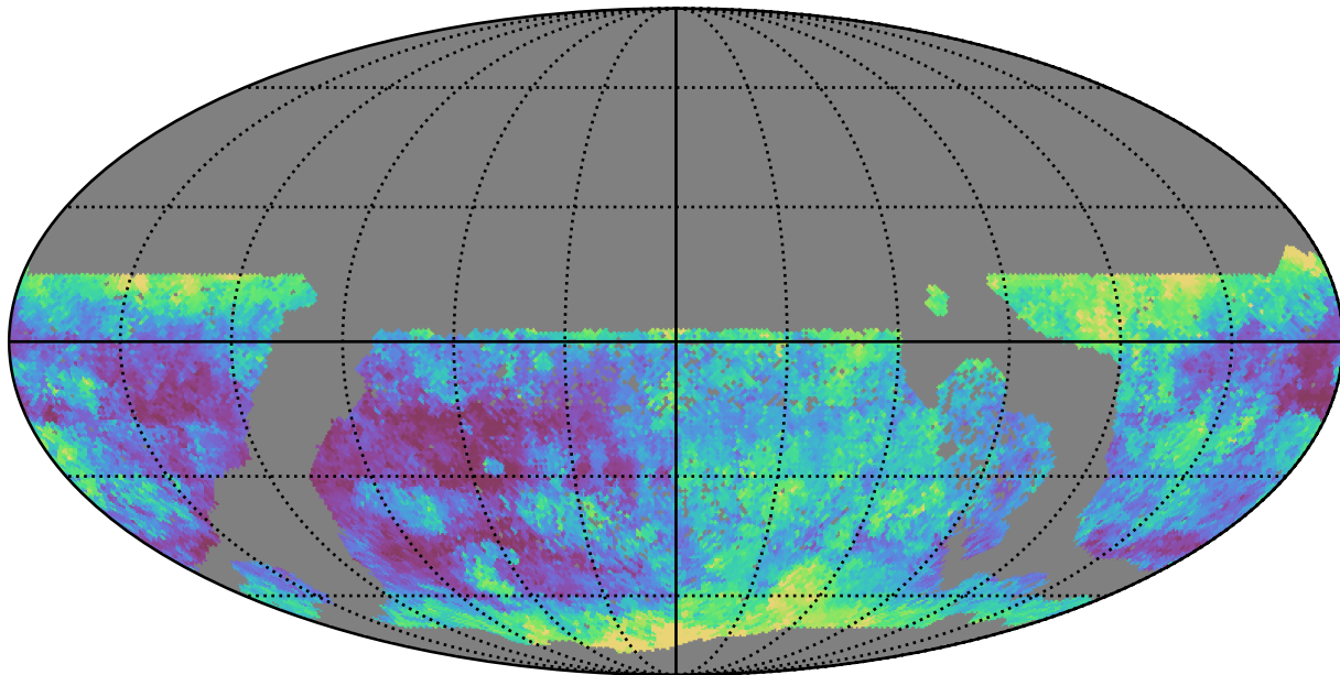
too_elab_r128_d2_griz_v3.4_10yrs WFD g band: Median seeingEff
