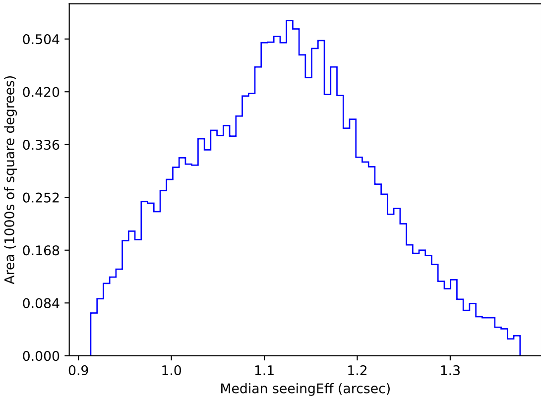
too_elab_r128_d2_griz_v3.4_10yrs WFD g band: Median seeingEff
