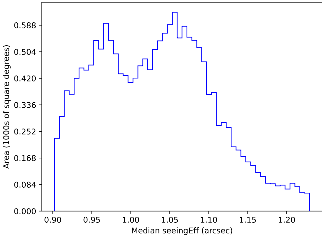
too_elab_r128_d2_griz_v3.4_10yrs WFD all bands: Median seeingEff
