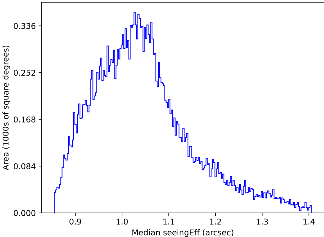
too_elab_r128_d2_griz_v3.4_10yrs All sky z band: Median seeingEff
