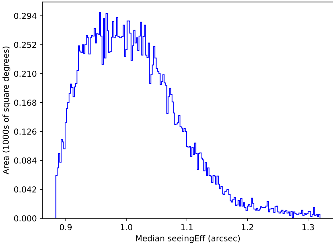
too_elab_r128_d2_griz_v3.4_10yrs All sky y band: Median seeingEff
