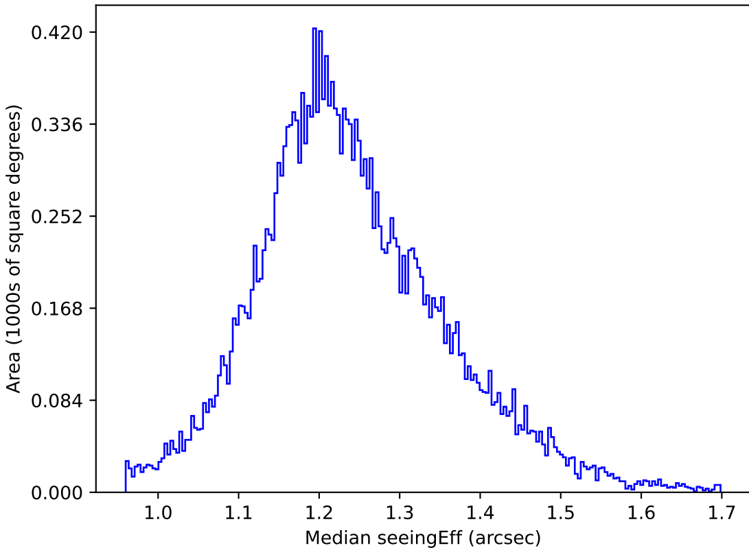
too_elab_r128_d2_griz_v3.4_10yrs All sky u band: Median seeingEff
