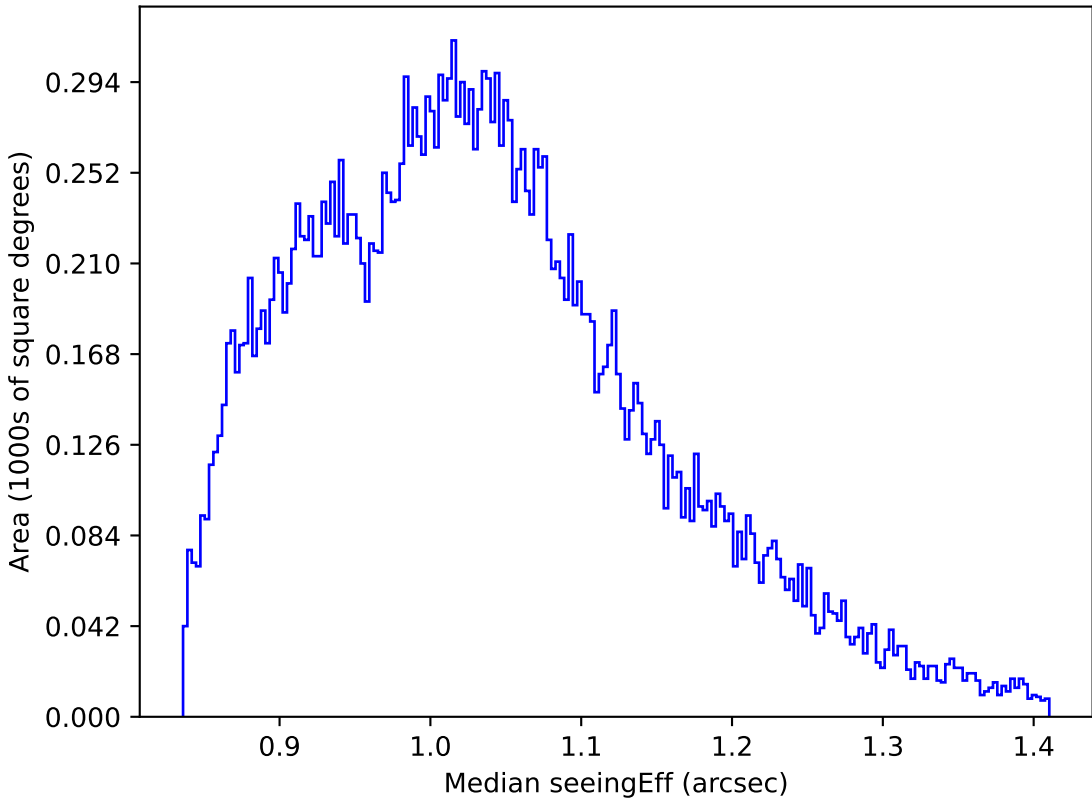
too_elab_r128_d2_griz_v3.4_10yrs All sky i band: Median seeingEff
