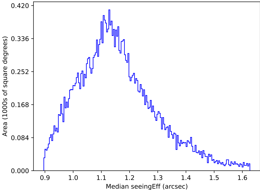
too_elab_r128_d2_griz_v3.4_10yrs All sky g band: Median seeingEff
