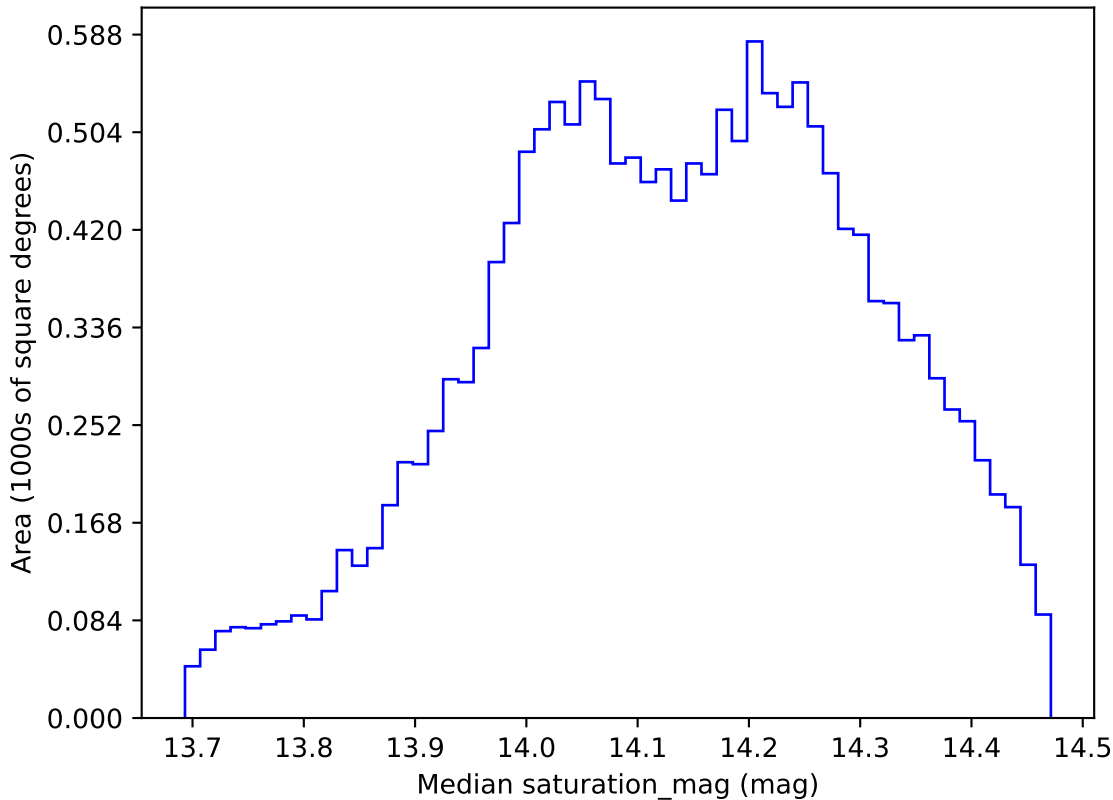
too_elab_r128_d2_griz_v3.4_10yrs WFD all bands: Median saturation_mag
