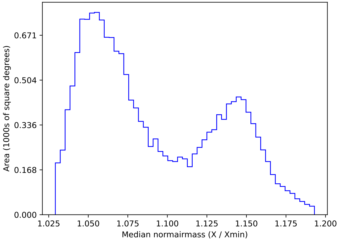
too_elab_r128_d2_griz_v3.4_10yrs WFD y band: Median normairmass
