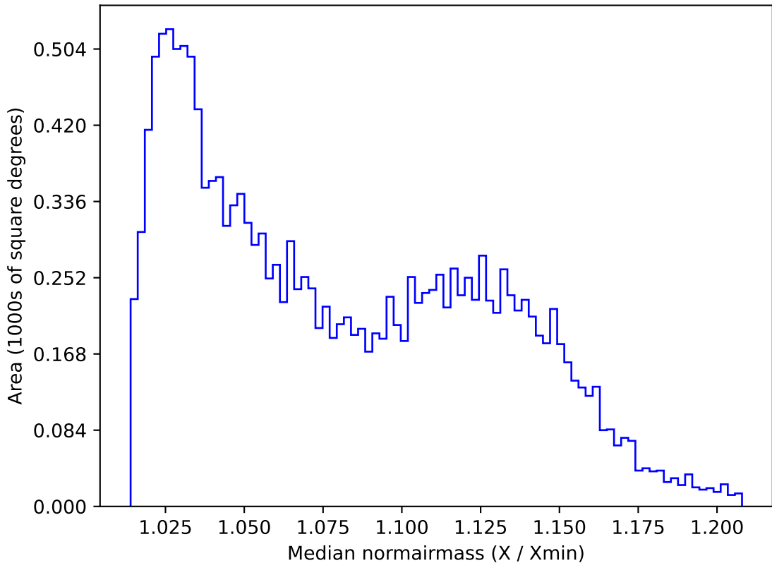
too_elab_r128_d2_griz_v3.4_10yrs WFD u band: Median normairmass
