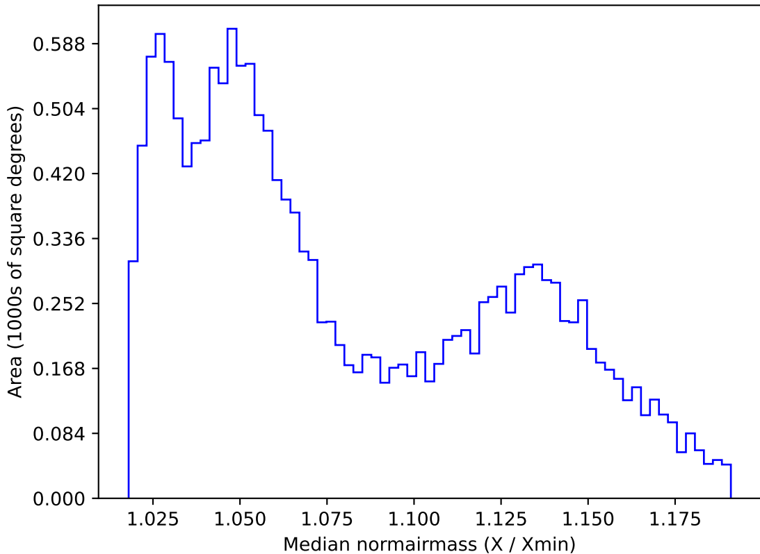
too_elab_r128_d2_griz_v3.4_10yrs WFD r band: Median normairmass
