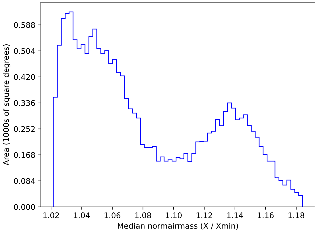
too_elab_r128_d2_griz_v3.4_10yrs WFD i band: Median normairmass
