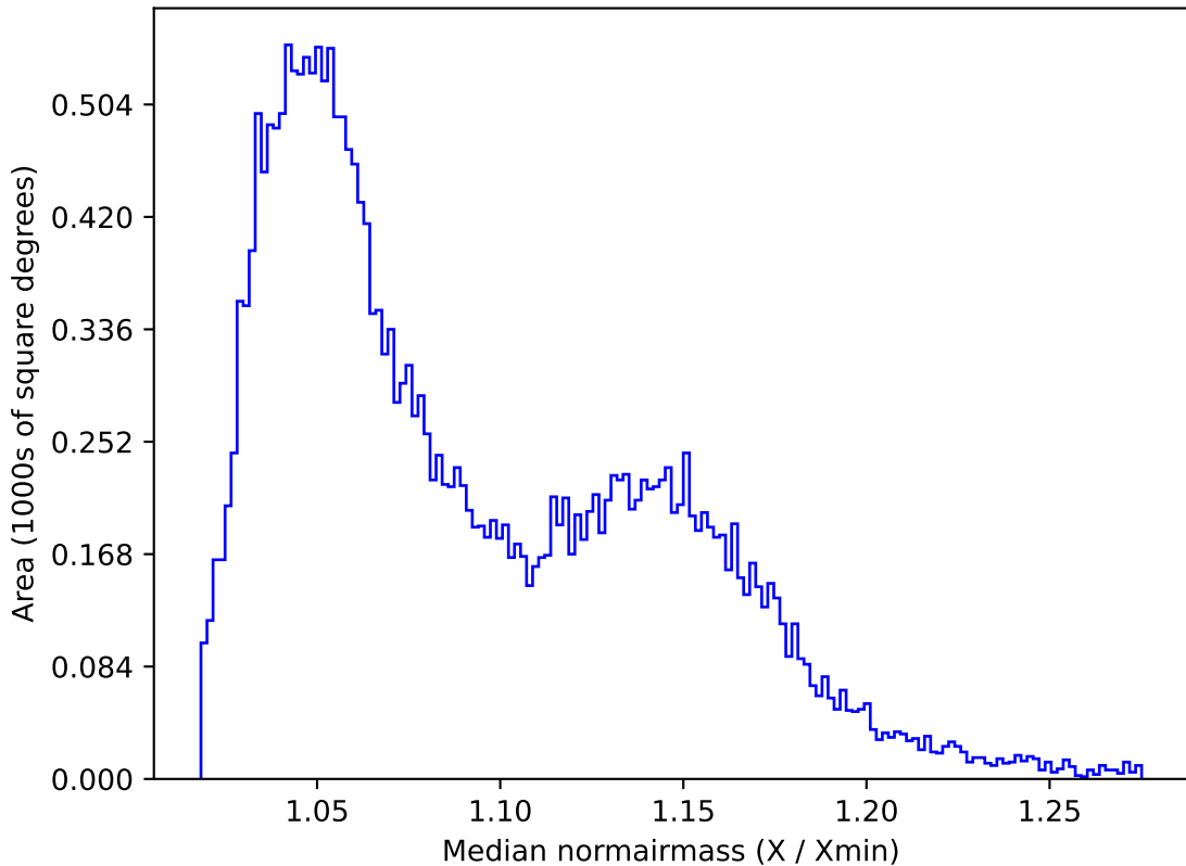
too_elab_r128_d2_griz_v3.4_10yrs All sky z band: Median normairmass
