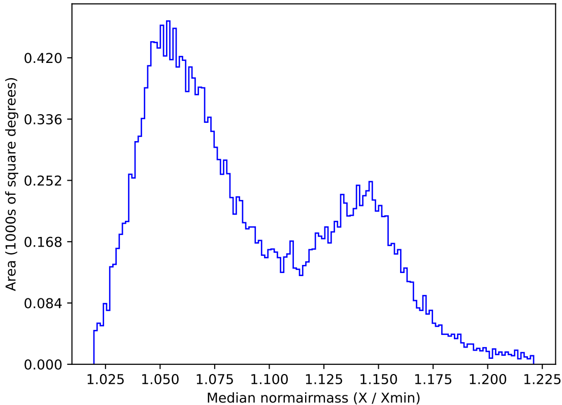
too_elab_r128_d2_griz_v3.4_10yrs All sky y band: Median normairmass
