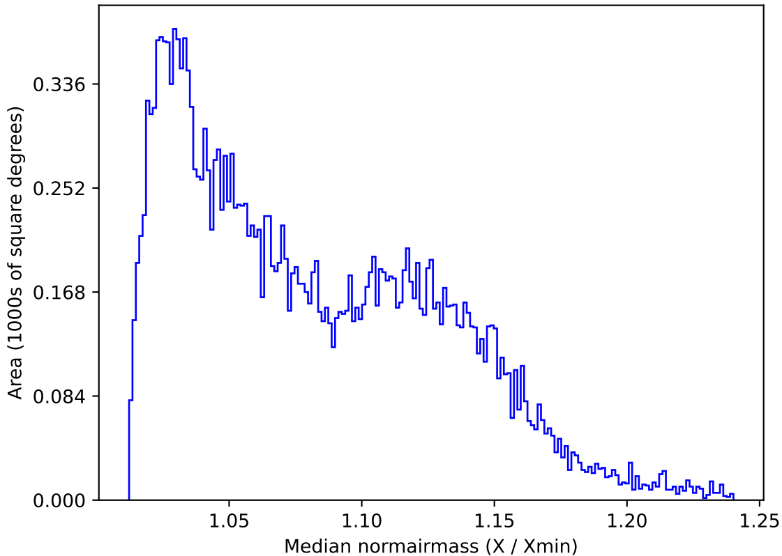
too_elab_r128_d2_griz_v3.4_10yrs All sky u band: Median normairmass
